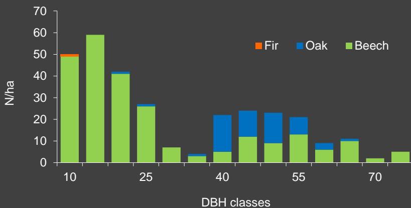
DBH distribution
